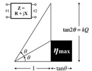
Fig.1: Wireless power transfer system black-box model and k-Q product chart
