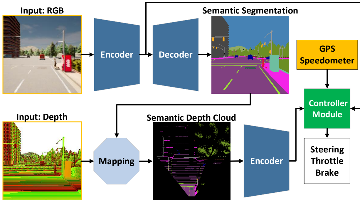
Caption: The AI model architecture is composed of the perception module (blue) and the controller module (green). The perception module is responsible for perceiving the environment based on the observation data provided by an RGBD camera. Meanwhile, the controller module is responsible for decoding the extracted information to estimate the degree of steering, throttle, and braking.
