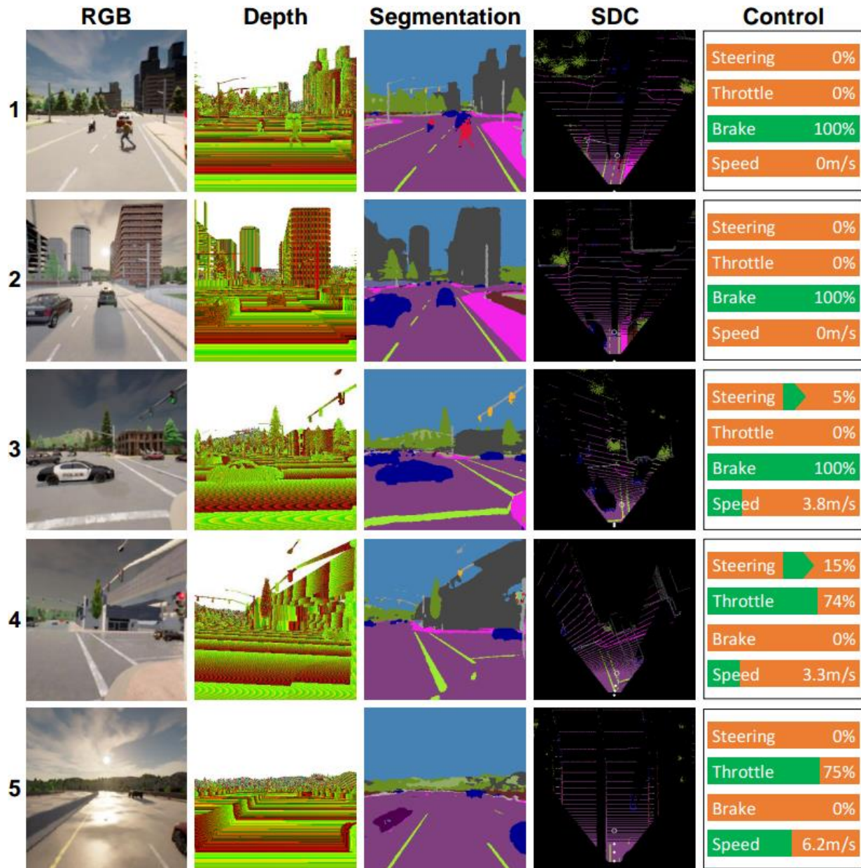
Caption: Some driving records made by the AI model. Columns (from left to right): color image, depth image, semantic segmentation result, birds-eye-view (BEV) map, control command. The weather and time for each scene are as follows: (1) clear noon, (2) cloudy sunset, (3) mid rainy noon, (4) hard rain sunset, (5) wet sunset.
