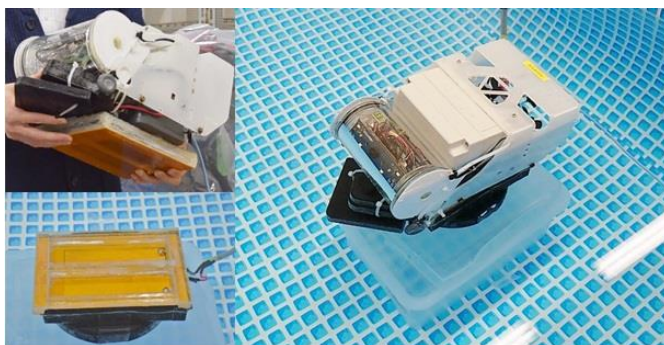
Caption: Underwater drone (top left), power supply station (bottom left), drone parked on the power supply station installed on the ocean floor for battery charging (right)
