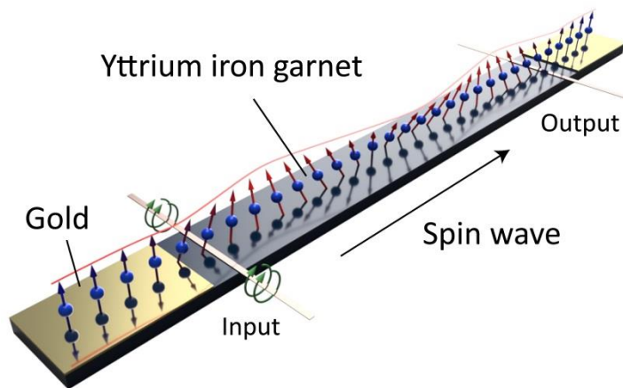
Caption: A magnetic oxide film treated with gold film capable of suppressing SW noise
