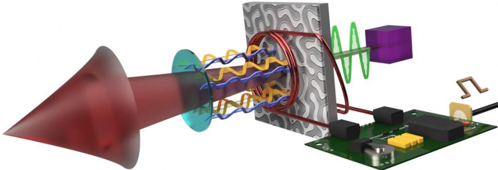
Caption: A pulsed output with a power of dozens of watts and a pulse width of 40 ns was obtained through an MO Q-switched laser controlled by labyrinth-shaped magnetic domains.
