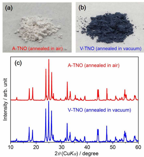
Figure 1: Photos of TNO annealed in air (A-TNO) (a) and vacuum (V-TNO) (b). X-ray diffraction patterns for both samples is also shown in (c).
