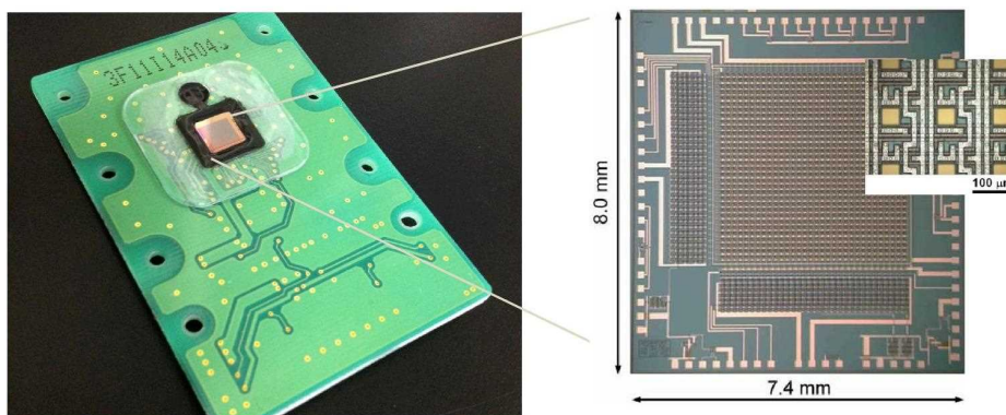
Fig. 1 Semiconductor image sensor (128 pixels × 128 pixels)
