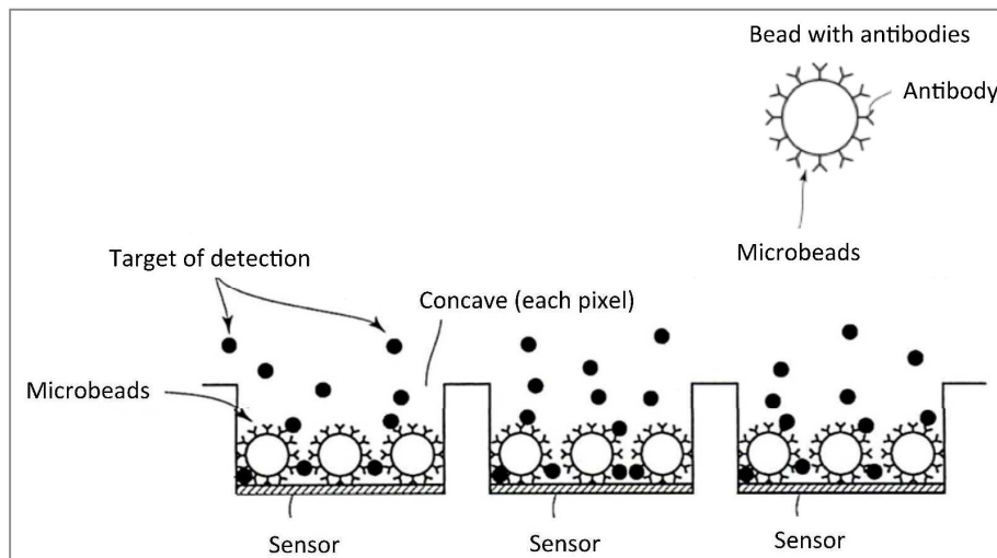
Fig. 2 Schematic illustration of microbeads with antibodies on sensors (Patent application filed)
