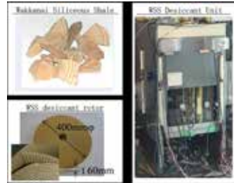
Pictures of WSS desiccant rotor and ventilation unit
