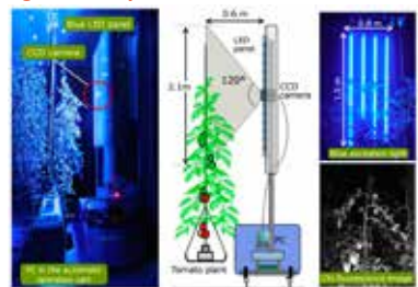
Chlorophyll fluorescence imaging robot for plant health diagnosis
