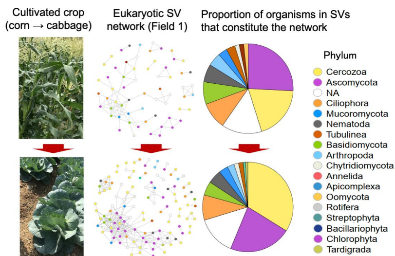
Figure: Network analysis of eukaryotic SVs in Field 1 under crop rotation
